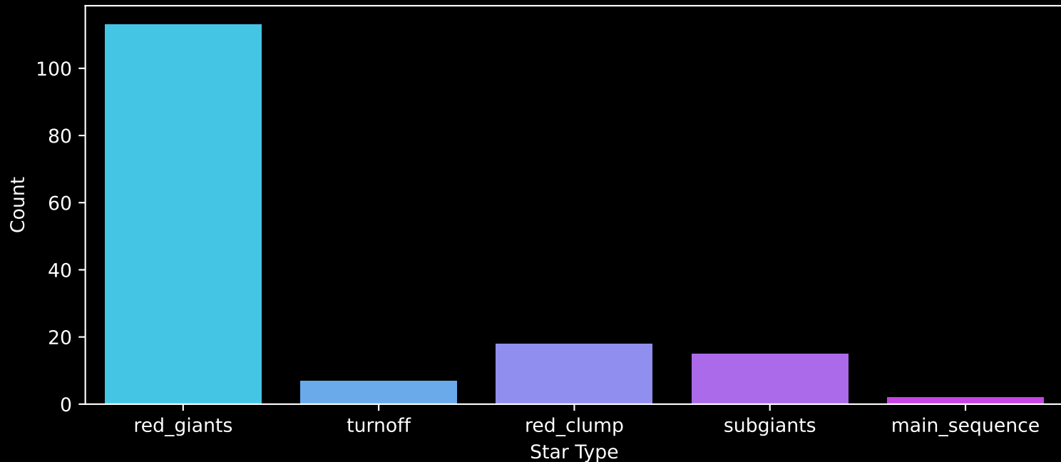
APOGEE DR17 Field: [068+04] Count plot of Star Type
