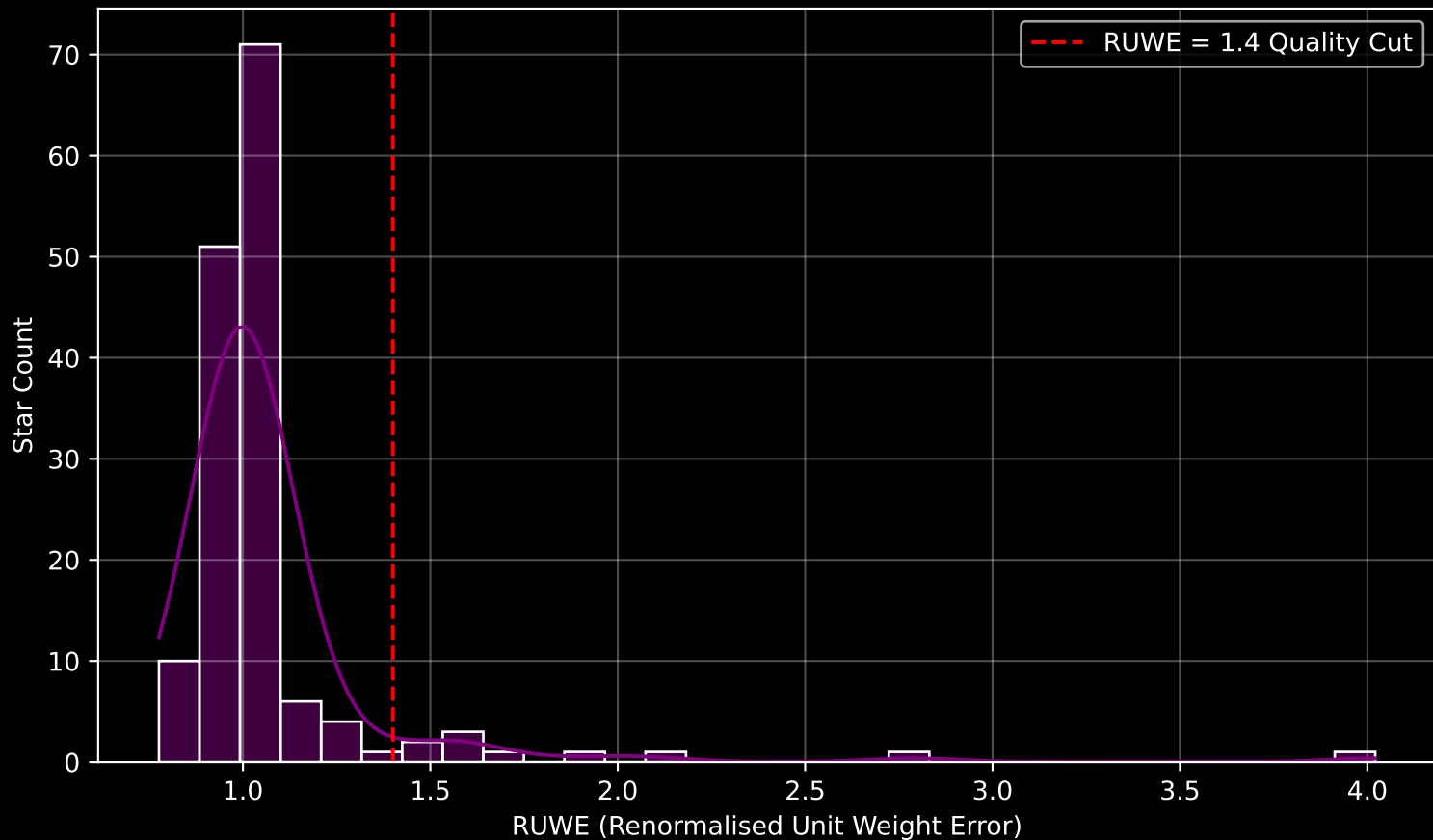
GAPOGEE DR17 Field [068+04] RUWE Distribution (n= 153)
