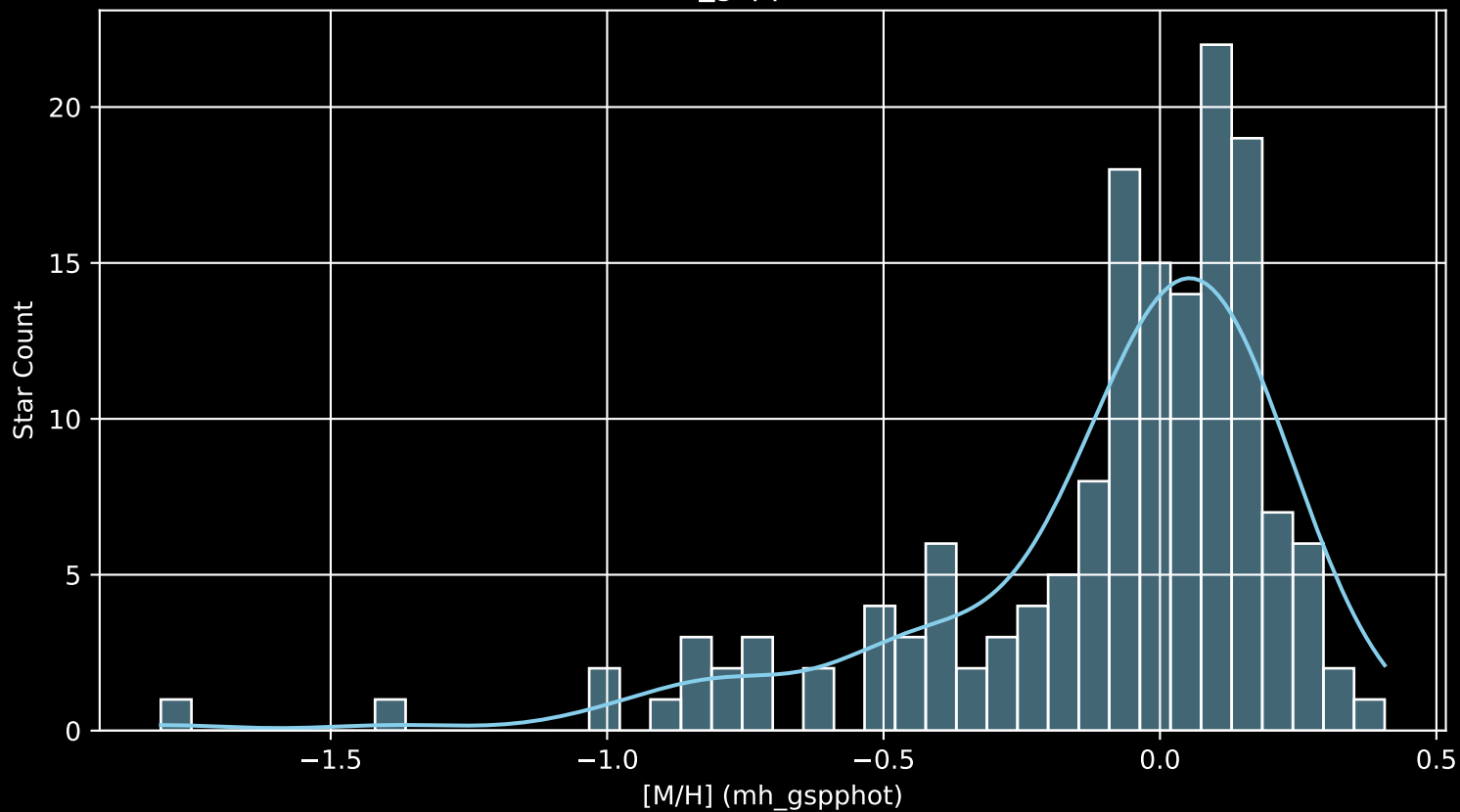
APOGEE DR17 Field: [068+04 [M/H] (mh_gspphot) (n= 154)
