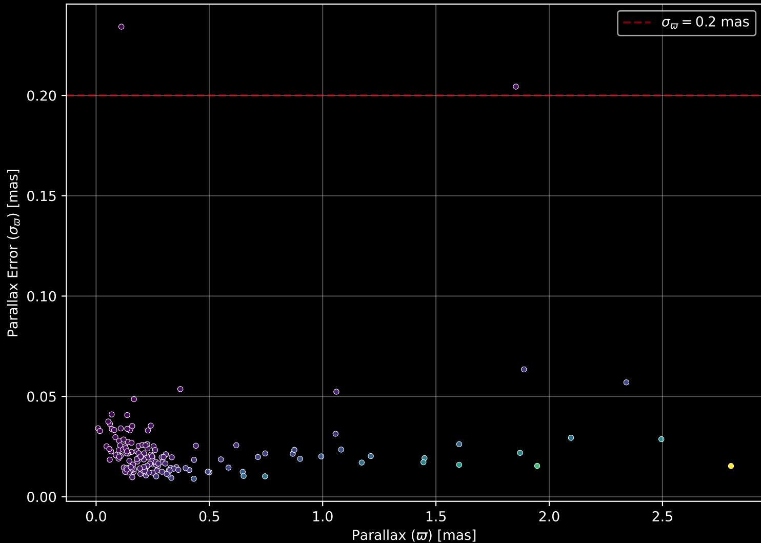
APOGEE DR17 Field: [068+04] Parallax Quality (n= 155)
