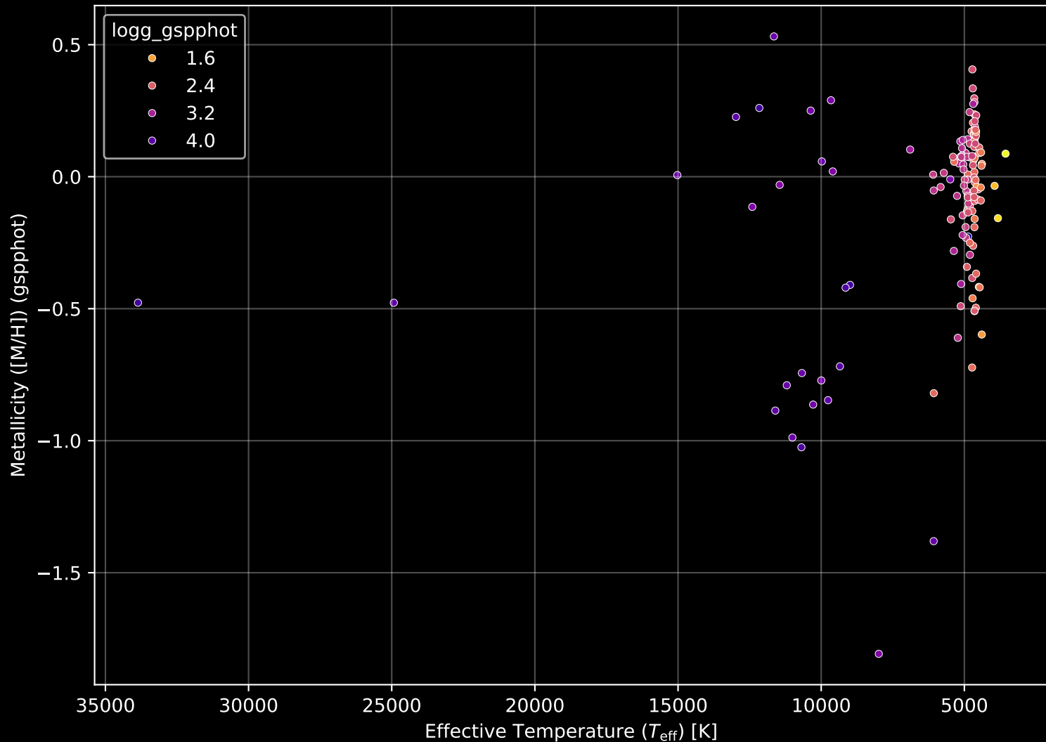
APOGEE DR17 Field: [068+04] Stellar Population Parameters (n= 155)
