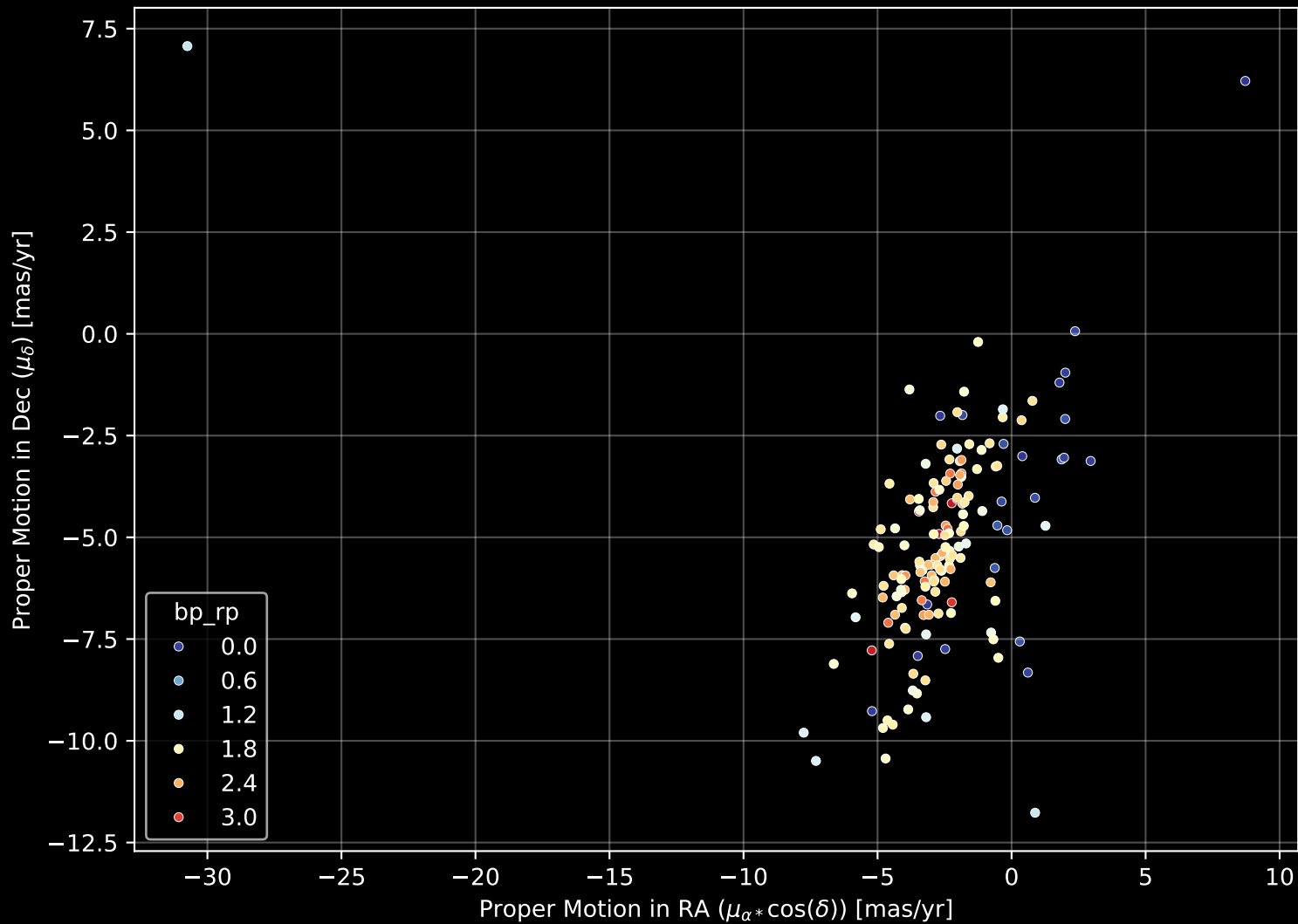
APOGEE DR17 Field: [068+04] Proper Motion Diagram (n= 155)
